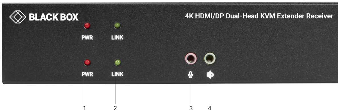
FIGURE 2-12. DUAL-HEAD RECEIVER FRONT PANEL
