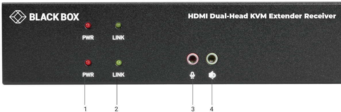
FIGURE 2-11. DUAL-HEAD RECEIVER FRONT PANEL
