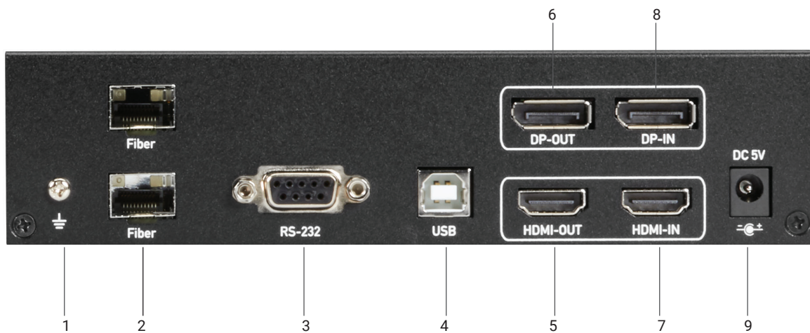
FIGURE 2-9. HDMI/DP DUAL-HEAD FIBER TRANSMITTER BACK PANEL
