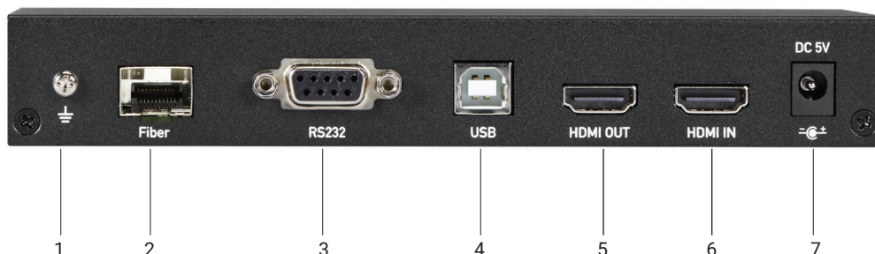
FIGURE 2-5. SINGLE-HEAD FIBER TRANSMITTER BACK PANEL
