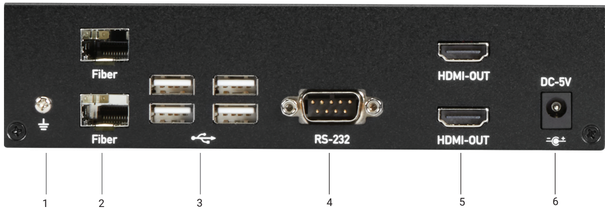
FIGURE 2-16. HDMI DUAL-HEAD FIBER RECEIVER BACK PANEL
