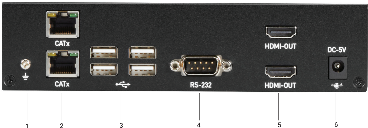
FIGURE 2-17. DUAL-HEAD CATX RECEIVER BACK PANEL
