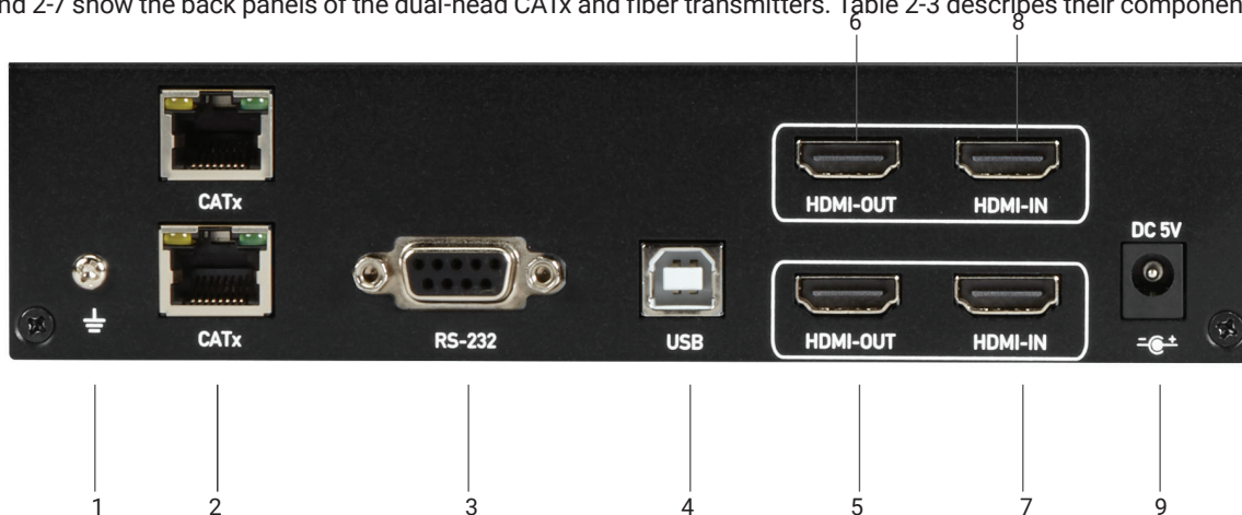
FIGURE 2-6. HDMI DUAL-HEAD CATX TRANSMITTER BACK PANEL
