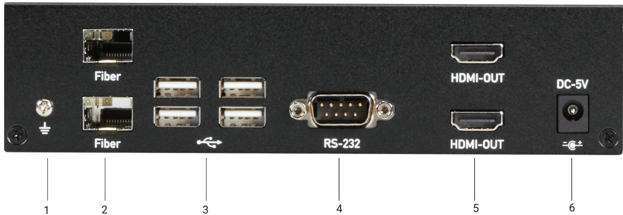
FIGURE 2-18. HDMI/DP DUAL-HEAD FIBER RECEIVER BACK PANEL
