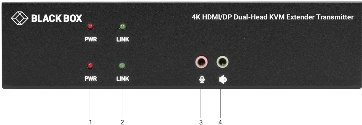
FIGURE 2-3. HDMI/DP DUAL-HEAD TRANSMITTER FRONT PANEL
