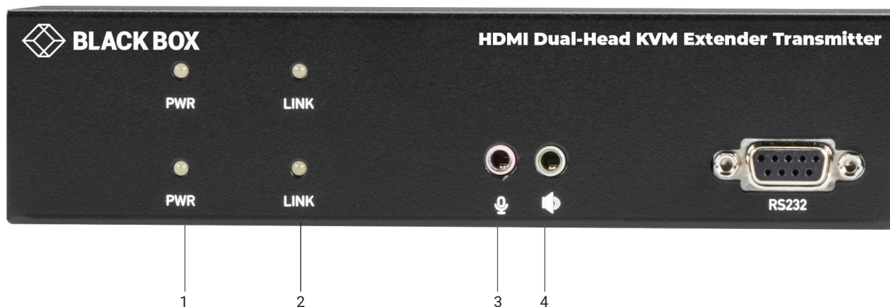
FIGURE 2-2. HDMI DUAL-HEAD TRANSMITTER FRONT PANEL
