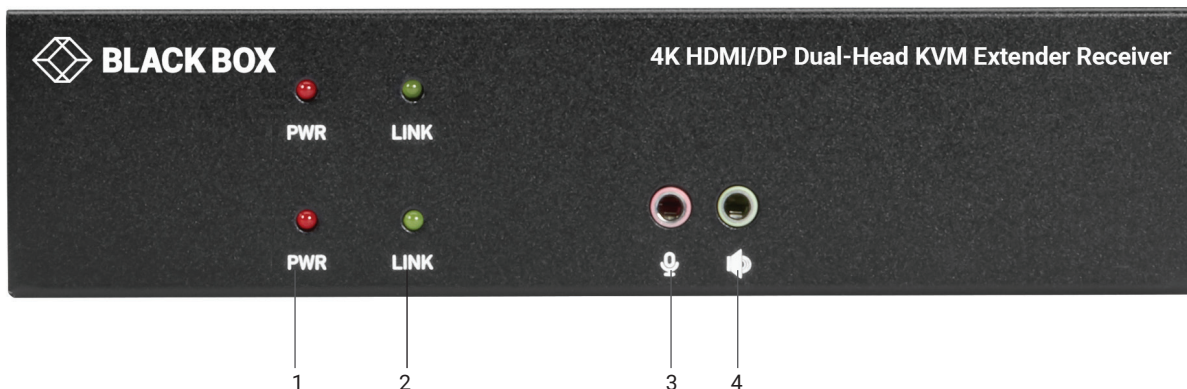
FIGURE 2-12. DUAL-HEAD RECEIVER FRONT PANEL
