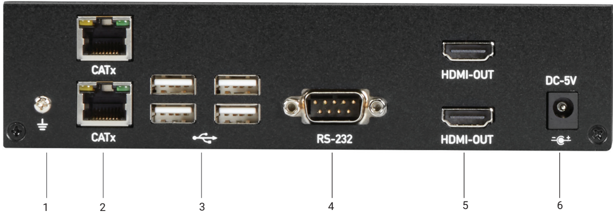
FIGURE 2-15. HDMI DUAL-HEAD CATX RECEIVER BACK PANEL
