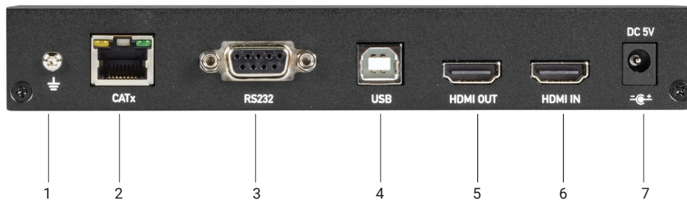
FIGURE 2-4. SINGLE-HEAD CATX TRANSMITTER BACK PANEL
