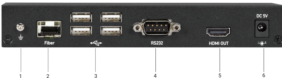
FIGURE 2-14. SINGLE-HEAD FIBER RECEIVER BACK PANEL
