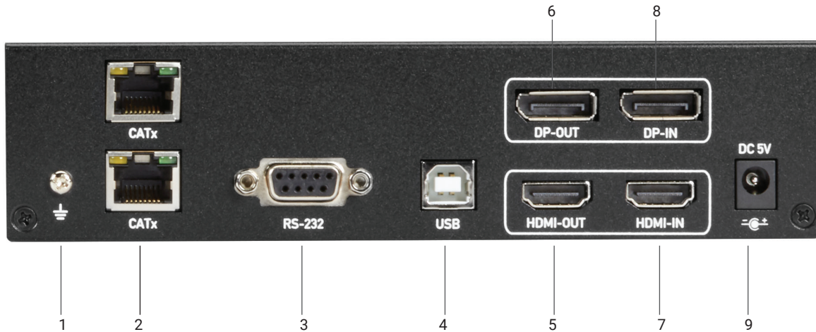
FIGURE 2-8. HDMI/DP DUAL-HEAD CATX TRANSMITTER BACK PANEL
