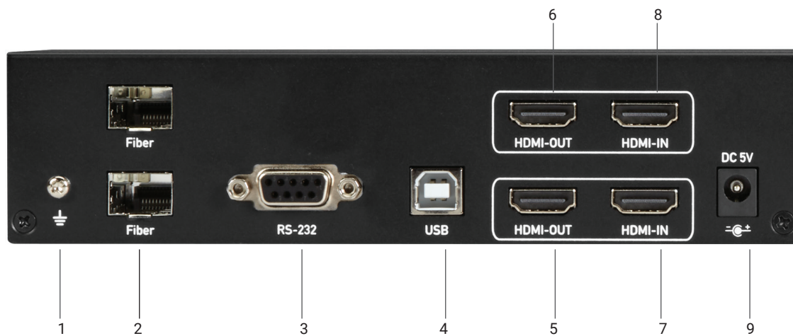
FIGURE 2-7. HDMI DUAL-HEAD FIBER TRANSMITTER BACK PANEL
