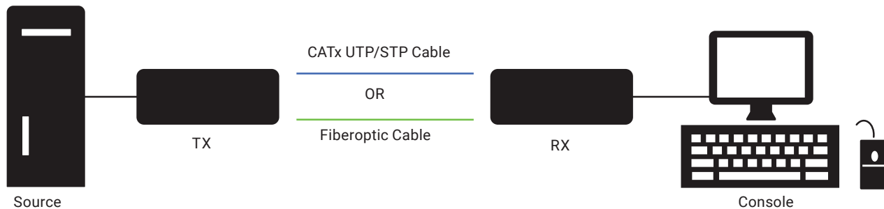
FIGURE 3-1. SINGLE-HEAD CONNECTION DIAGRAM
