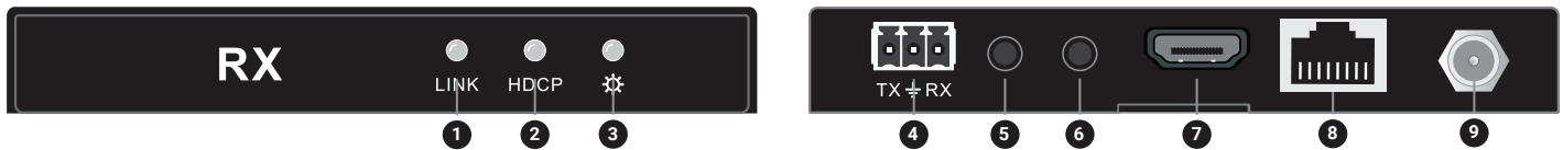
FIGURE 2-2. RECEIVER FRONT AND BACK PANELS
