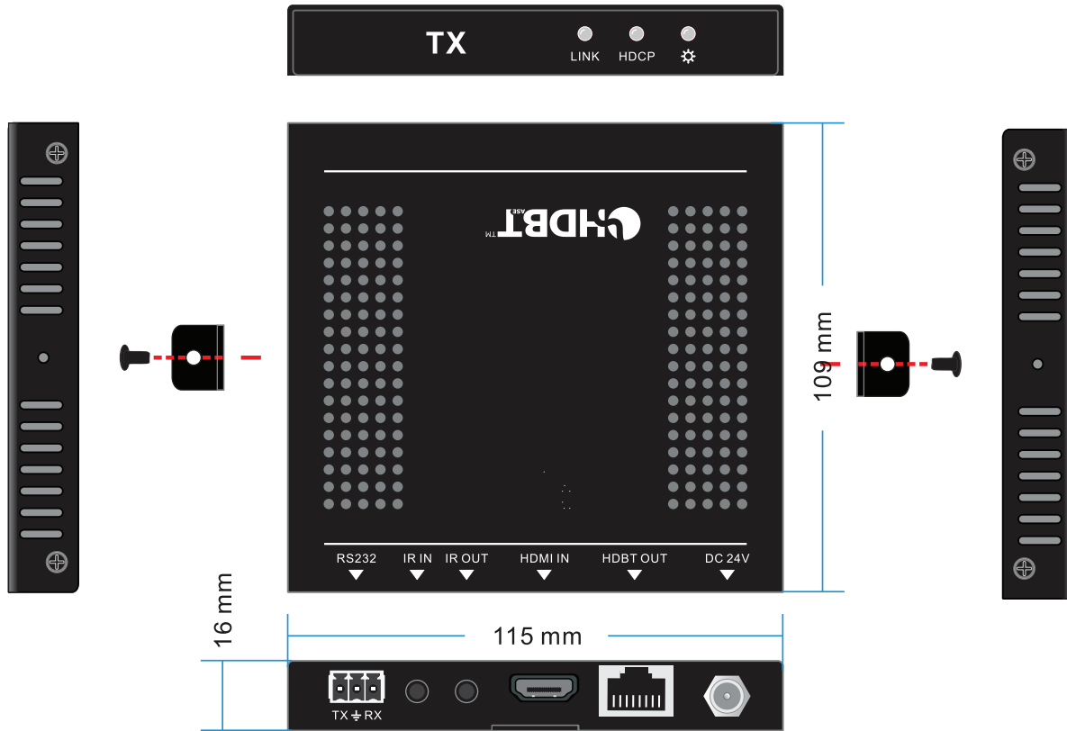
FIGURE 4-1. DIMENSIONAL DRAWING
