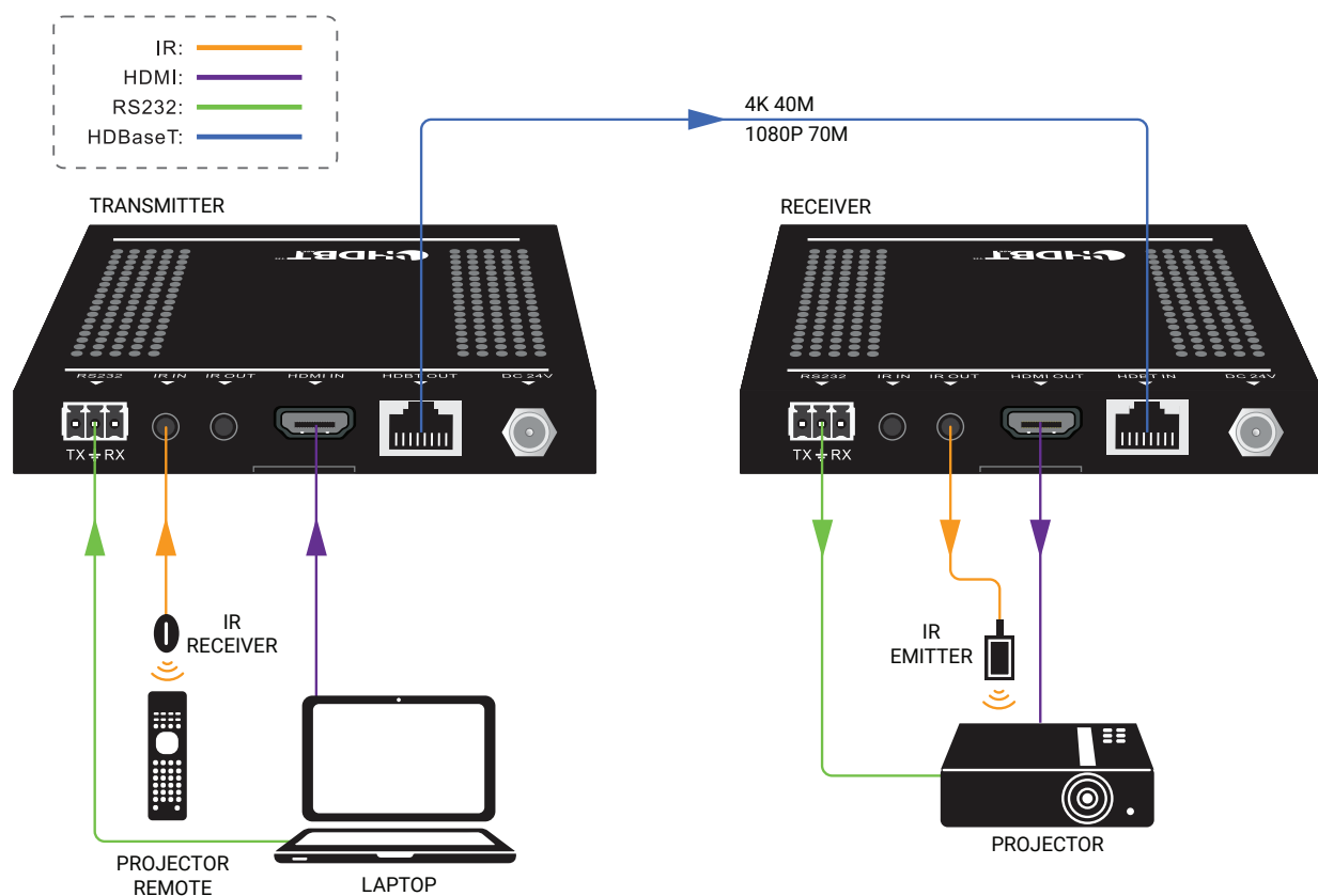
FIGURE 3-1. TYPICAL INSTALLATION
