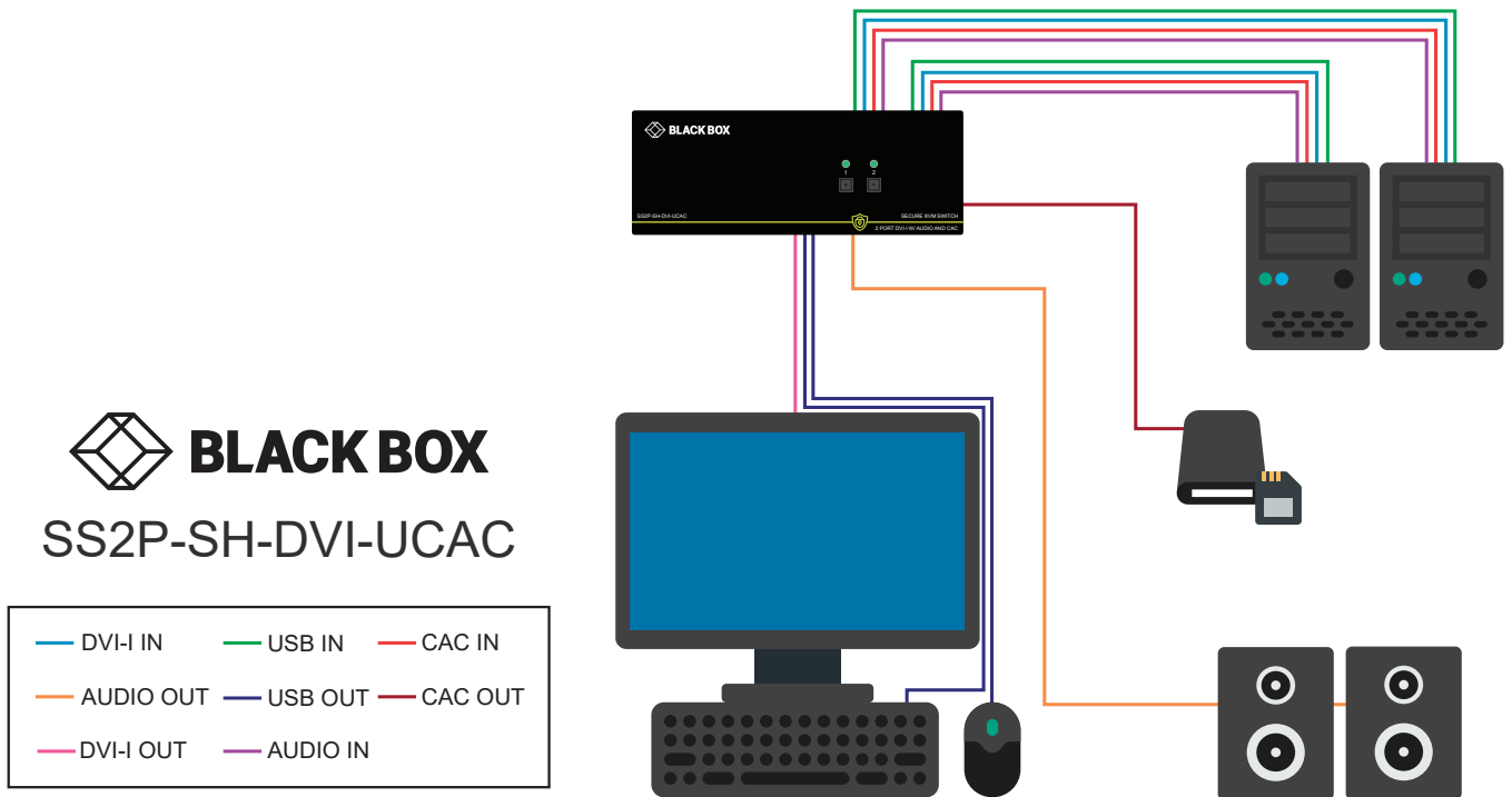
Figure 8-2 SS2P-SH-DVI-UCAC Shown
