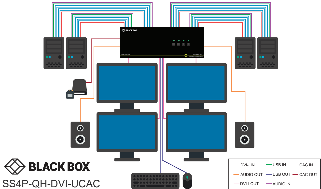
Figure 8-1 SS4P-QH-DVI-UCAC Shown
