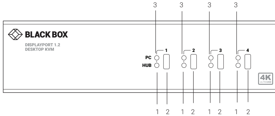
FIGURE 2-3. FRONT PANEL OF THE KV6224A-R2
