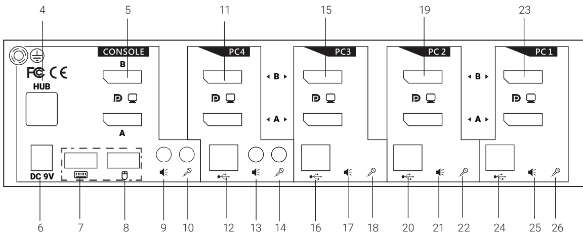
FIGURE 2-4. BACK PANEL OF THE KV6224A-R2
