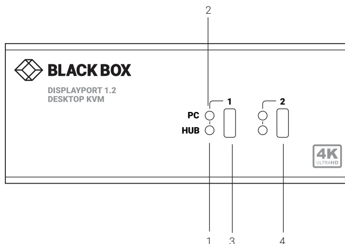
FIGURE 2-1. FRONT PANEL OF THE KV6222A-R2
