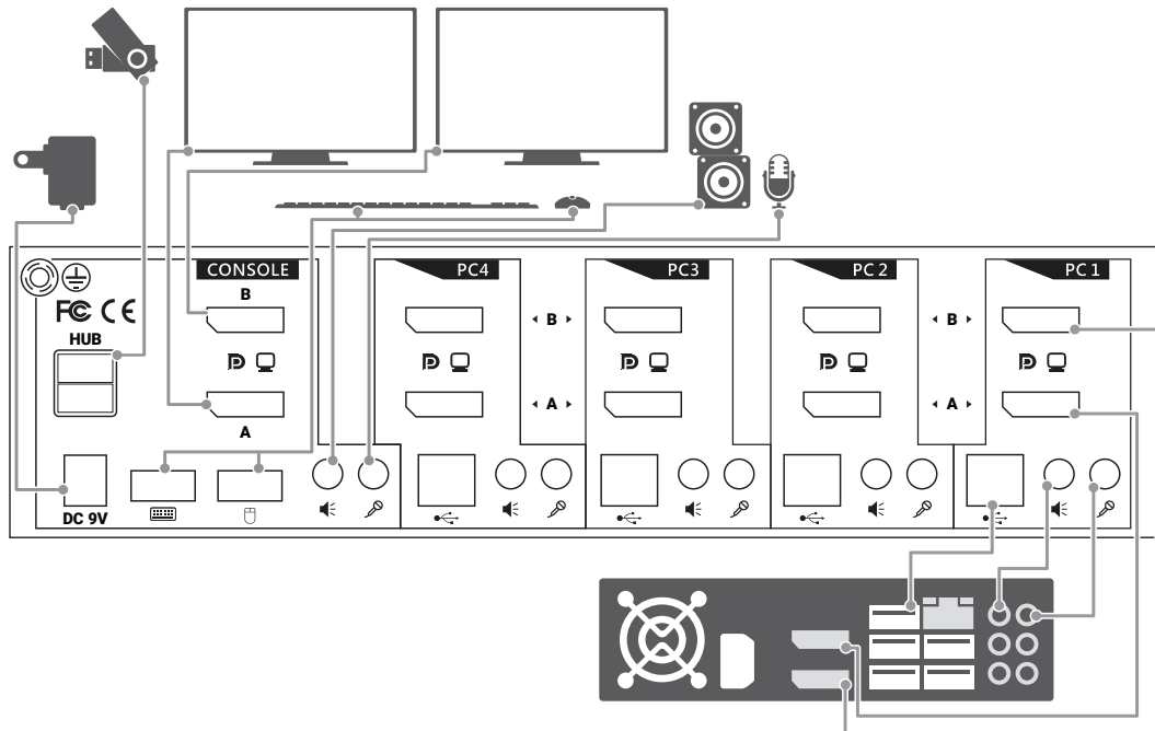
FIGURE 3-1. TYPICAL CONNECTIONS
