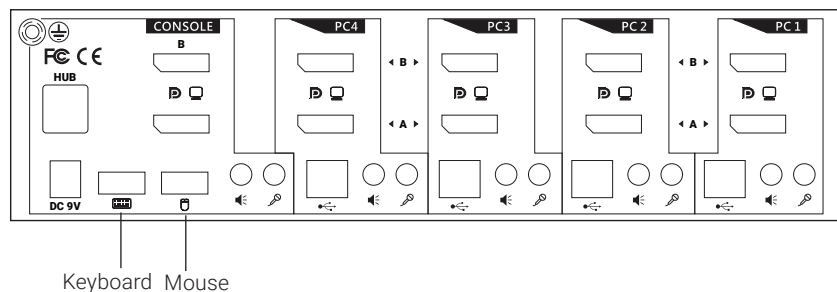
FIGURE 3-2. KEYBOARD AND MOUSE CONNECTIONS
